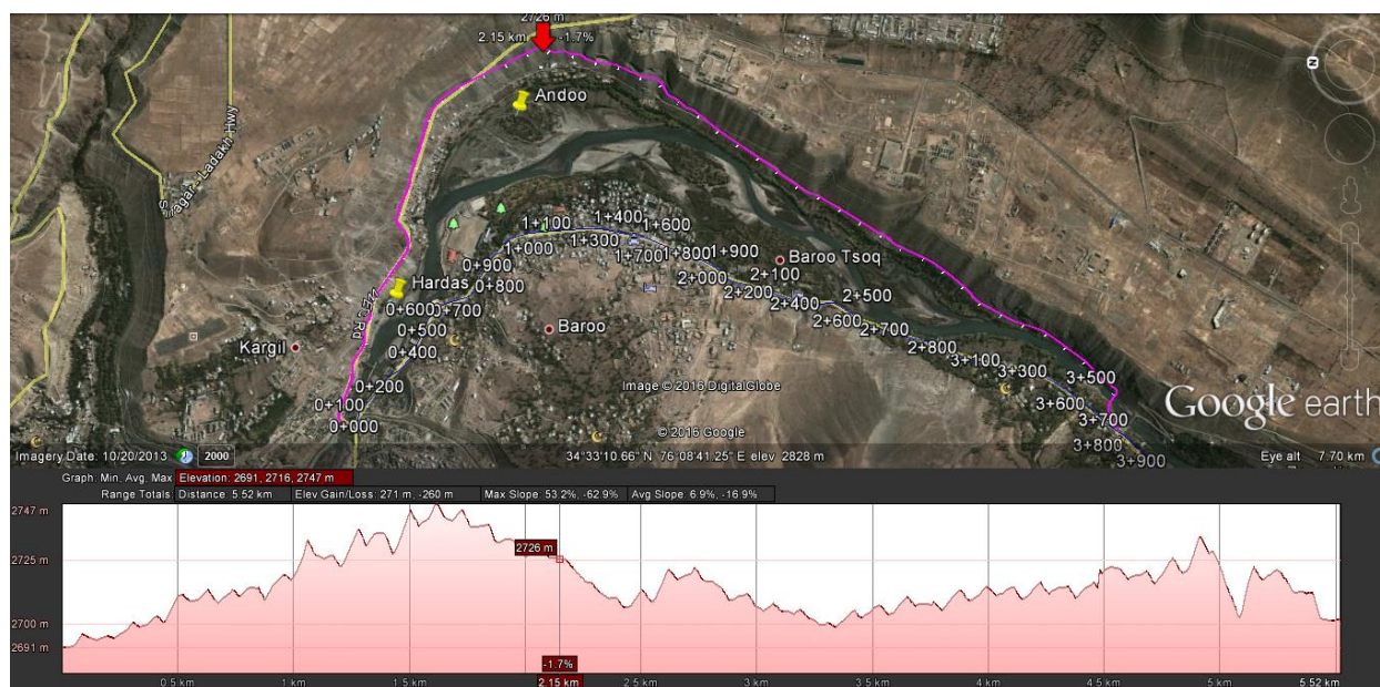
Figure 4.3: Proposed Kargil Bypass-Alternative-III
