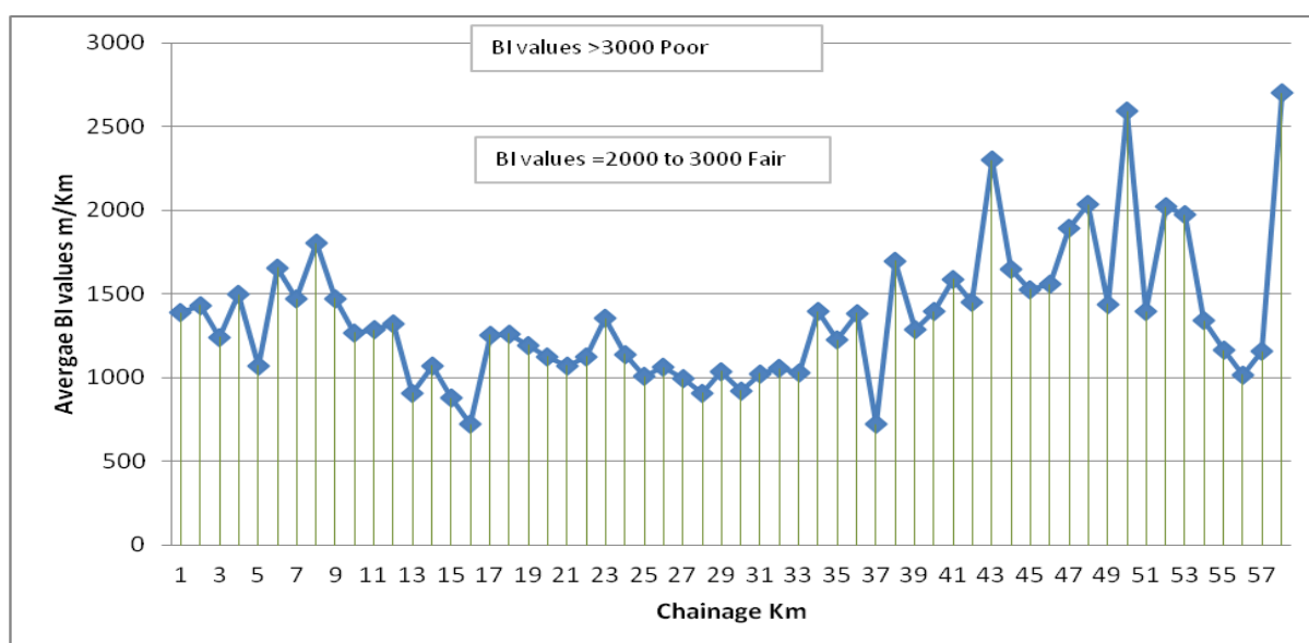
Figure 2.1: Roughness Values
