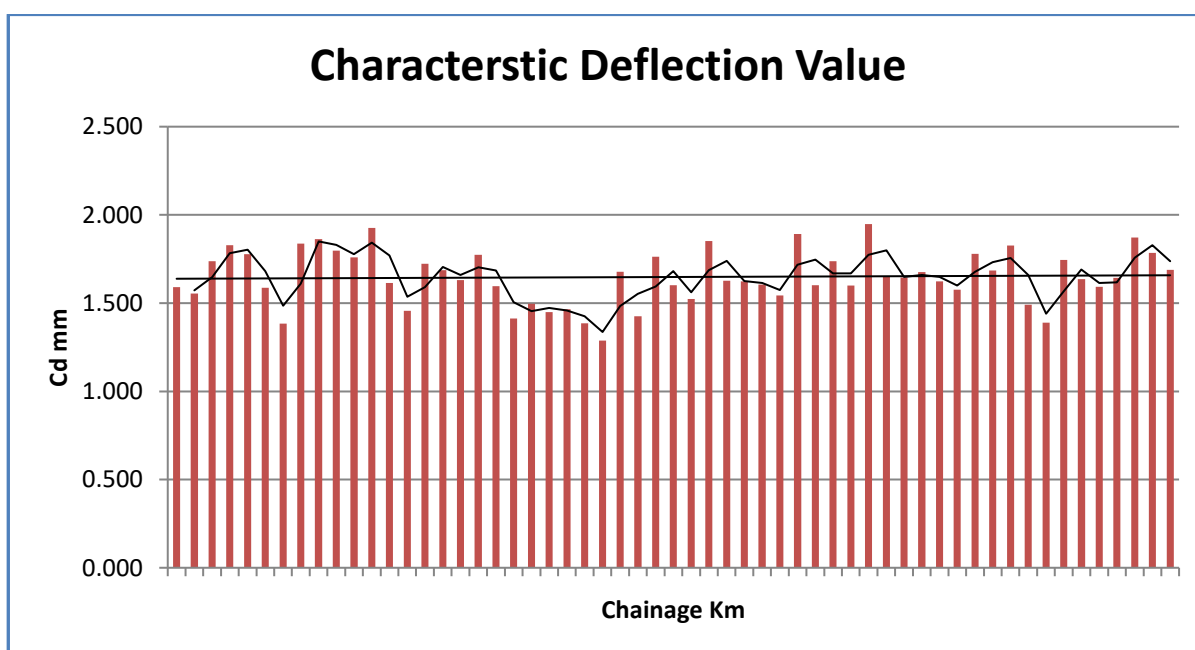
Figure 2.2: Characteristic Deflection along the Project Road
